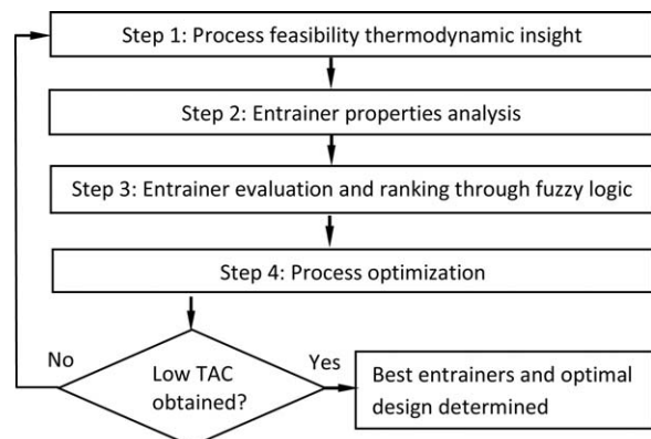
Figure 2. Block flow diagram of the proposed design method.
