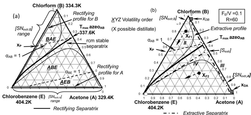
Figure 5. Thermodynamic principles for 1.0–2 case with chlorobenzene.
