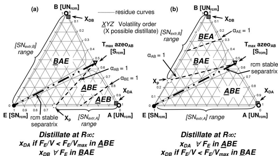
Figure 3. Thermodynamic features of 1.0-2 mixtures with respect to the separation of a maximum boiling azeotrope with a heavy entrainer.
